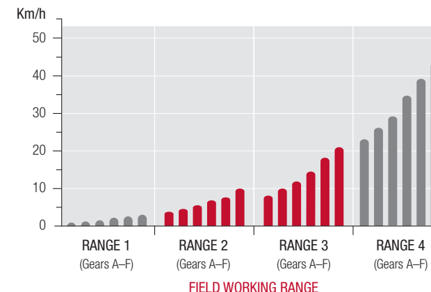
DYNA-6 TRANSMISSION
